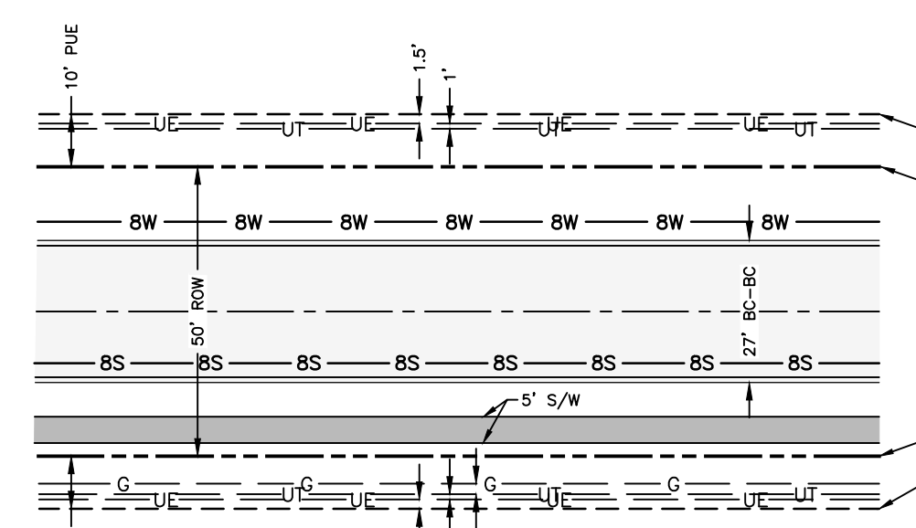
NOTE: This serves as a general guide only. Utility Company is to provide location of proposed electric, gas, and telecommunication lines.
